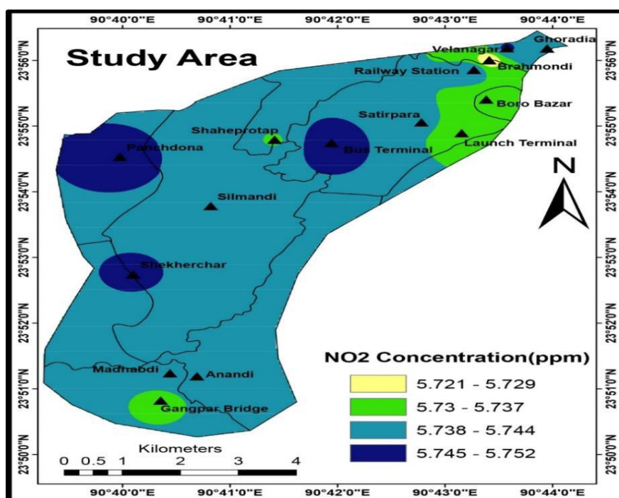
Fig. 6: Spatial distribution of NO 2 in the study area.
