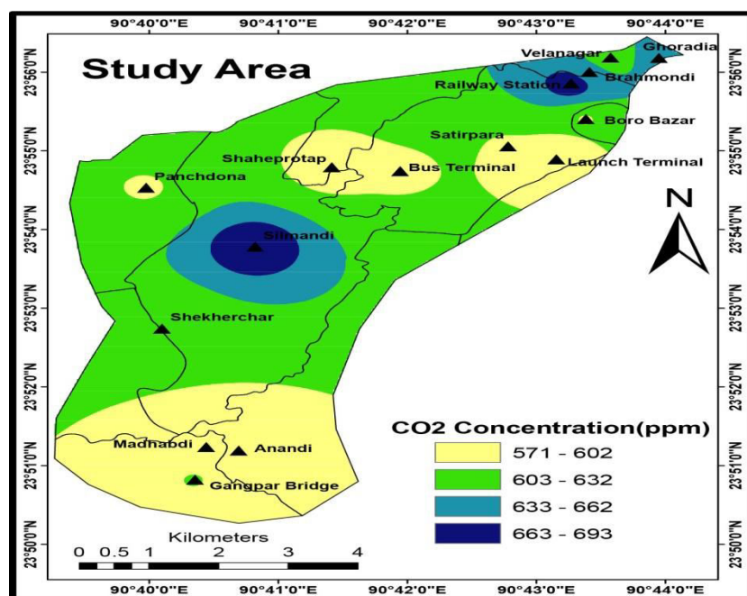
Fig. 8: Spatial distribution of CO 2 in the study area.
