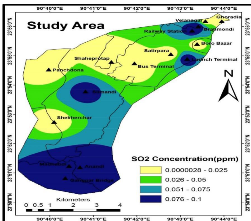
Fig. 7: Spatial distribution of SO 2 in the study area.
