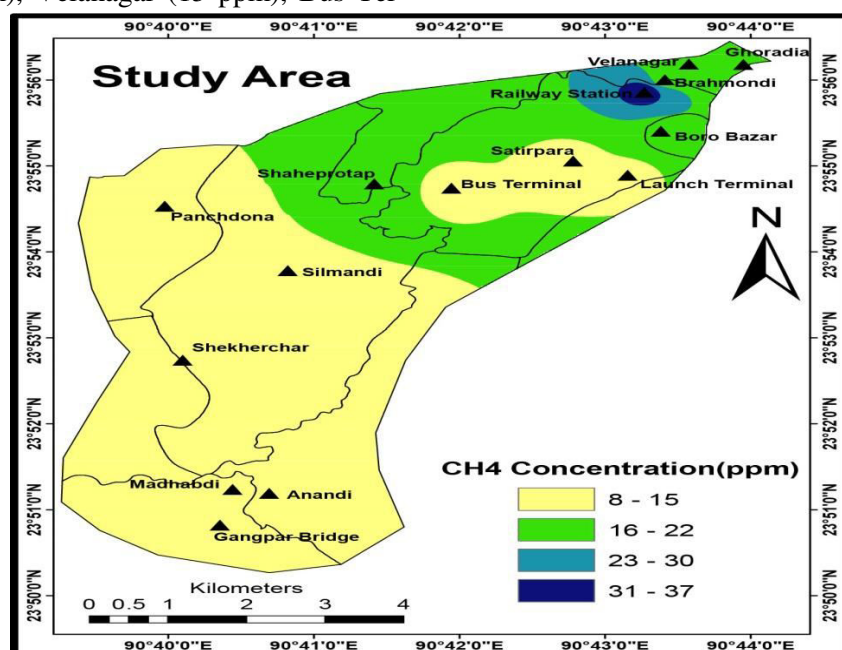
Fig. 9: Spatial distribution of CH 4 in the study area.
