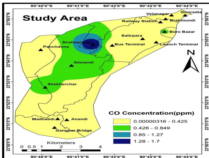
Fig. 5: Spatial distribution of CO in the study area.
