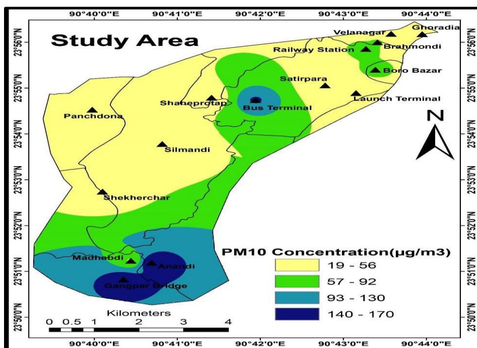
Fig. 4: Spatial distribution of PM 10 in the study area.
