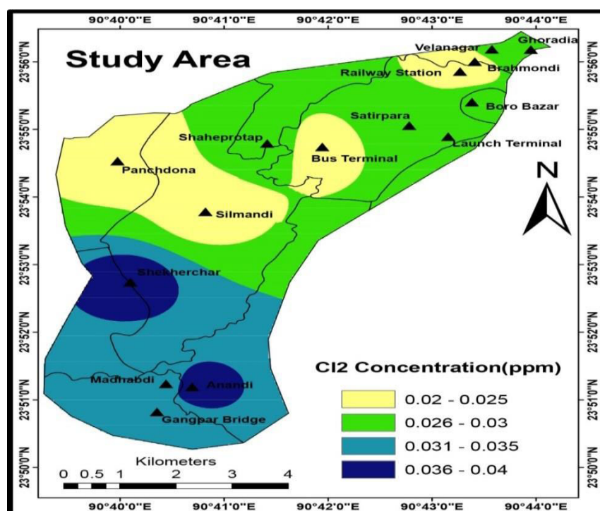
Fig. 10: Spatial distribution of \text{Cl}_2 in the study area.
