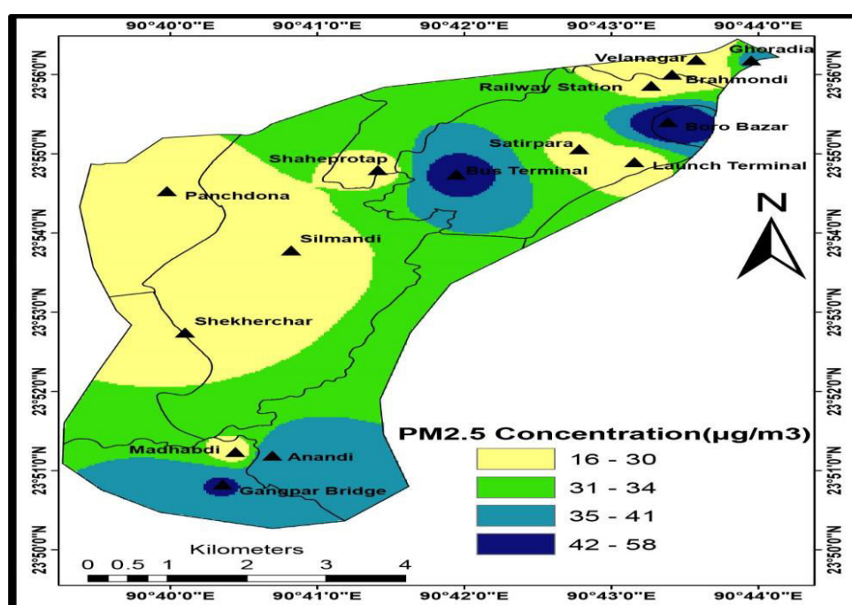
Fig. 3: Spatial distribution of \text{PM}_{2.5} in the study area.
